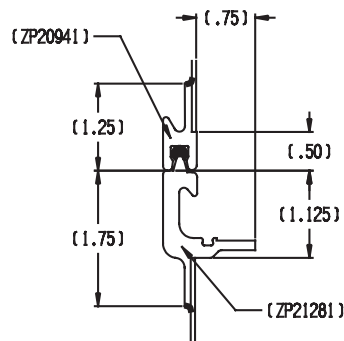
CLOSURE DETAIL
