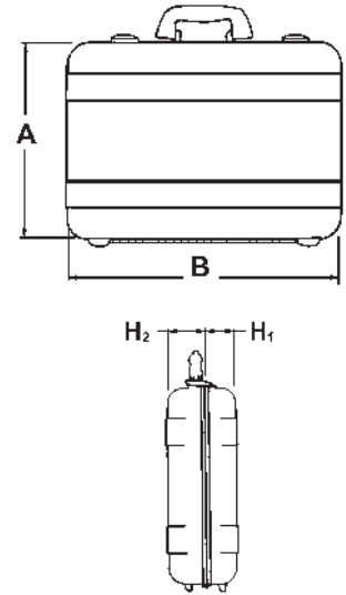
BASIC SHELL DIMENSIONS AND CASE SPECIFICATIONS
