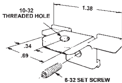
BRACKET FOR Z100X AND Z700X SERIES
